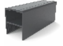
Tüp Motor Borusu Tube Motor Profile Profile Nr : 37115 Weight kg/m: 1 (72,3 x 2 mm)
