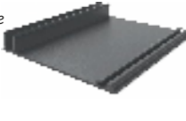
24mm Çekici Profili 24mm Attractive Profile Profile Nr : 37264 Weight kg/m: 0,782 (38,45 x 35 x 2,5mm)
