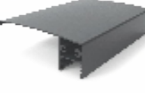
8mm Çekici Profili 8mm Attractive Profile Profile Nr : 37274 Weight kg/m: 0,847 (12,6 x 145 x 1,8 mm)
